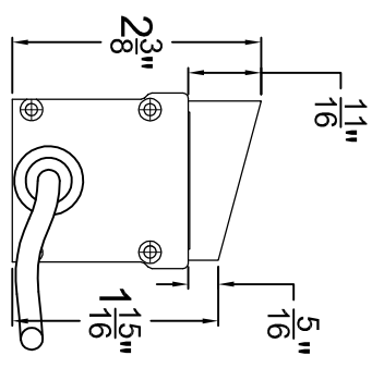
2 ELEVATION VIEW - LEFT SIDE ORIENTATION SCALE: 6" = 1'-0"
